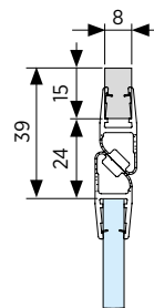
③ 45°-Profil 8x15 (rechts) 6 mm Glas Aluminium
