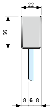
① Klemmprofil 6 mm Glas Aluminium
