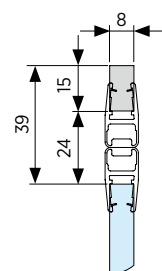
④ 0°-Profil 8x15 8 mm Glas Aluminium
